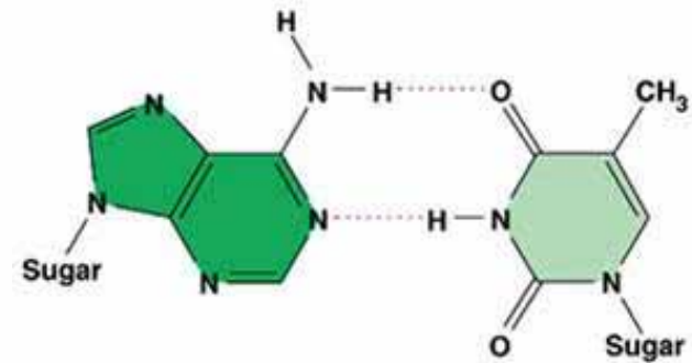
Adenine (A)
