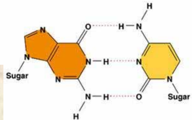
Guanine (G)
